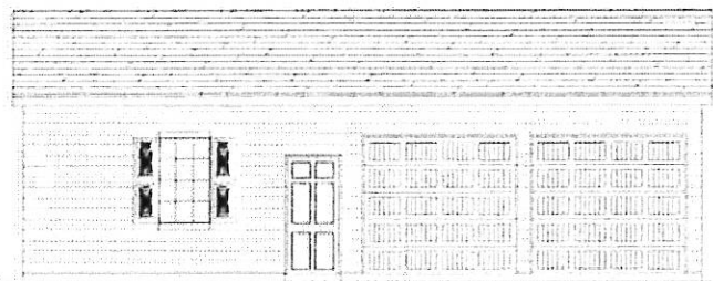
FRONT ELEVATION
