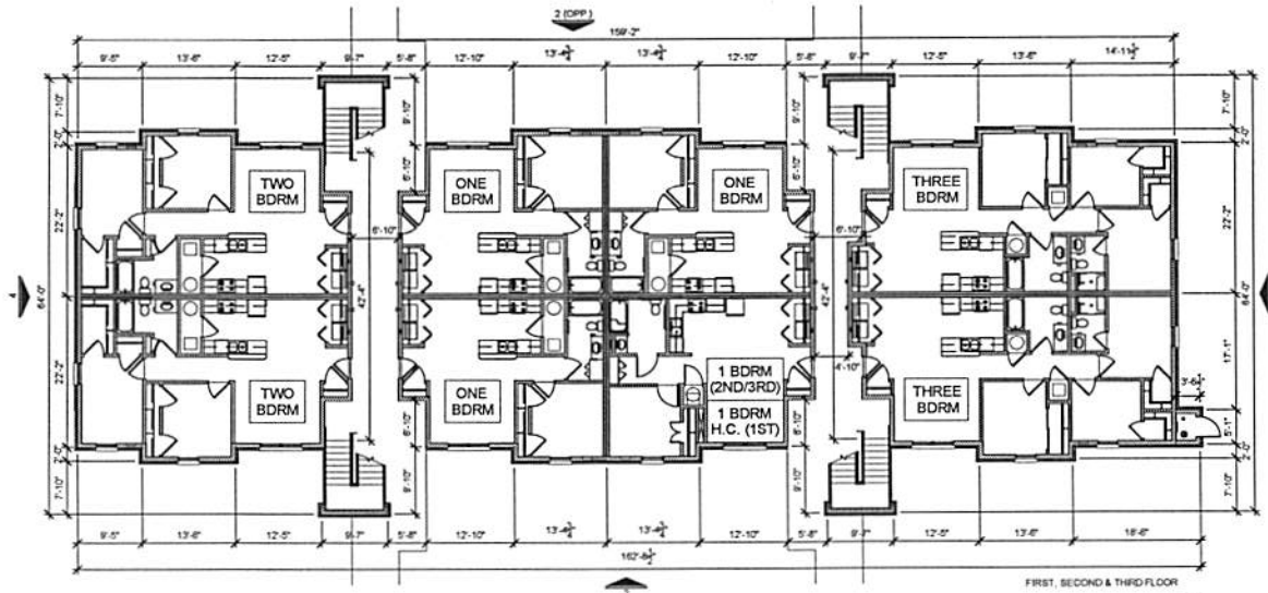
1 BUILDING A FLOOR PLAN SCALE: 0 5 10 20 40
