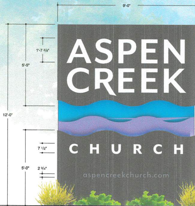
SOUTH ELEVATION VIEW
