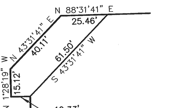
RESERVE AREA 'E' & UTILITY EASEMENT SCALE: 1"=30'
