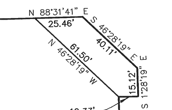
RESERVE AREA 'D' & UTILITY EASEMENT SCALE: 1"=30'
