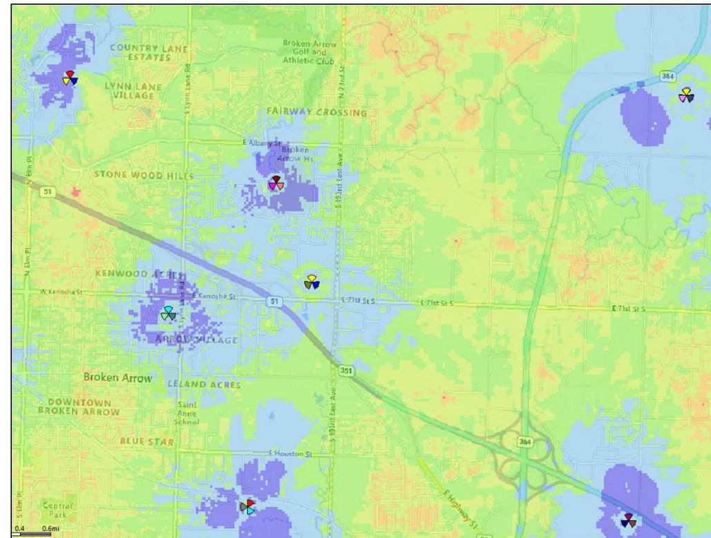
NSB Coverage: 155' RAD
