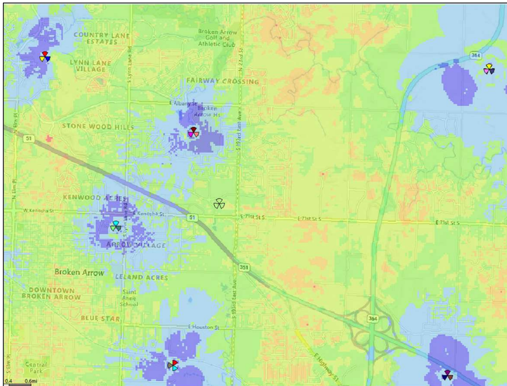
Existing Network Coverage
