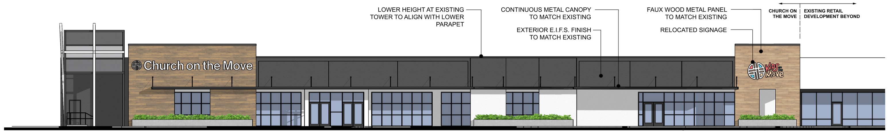
MAIN EXTERIOR ELEVATION
