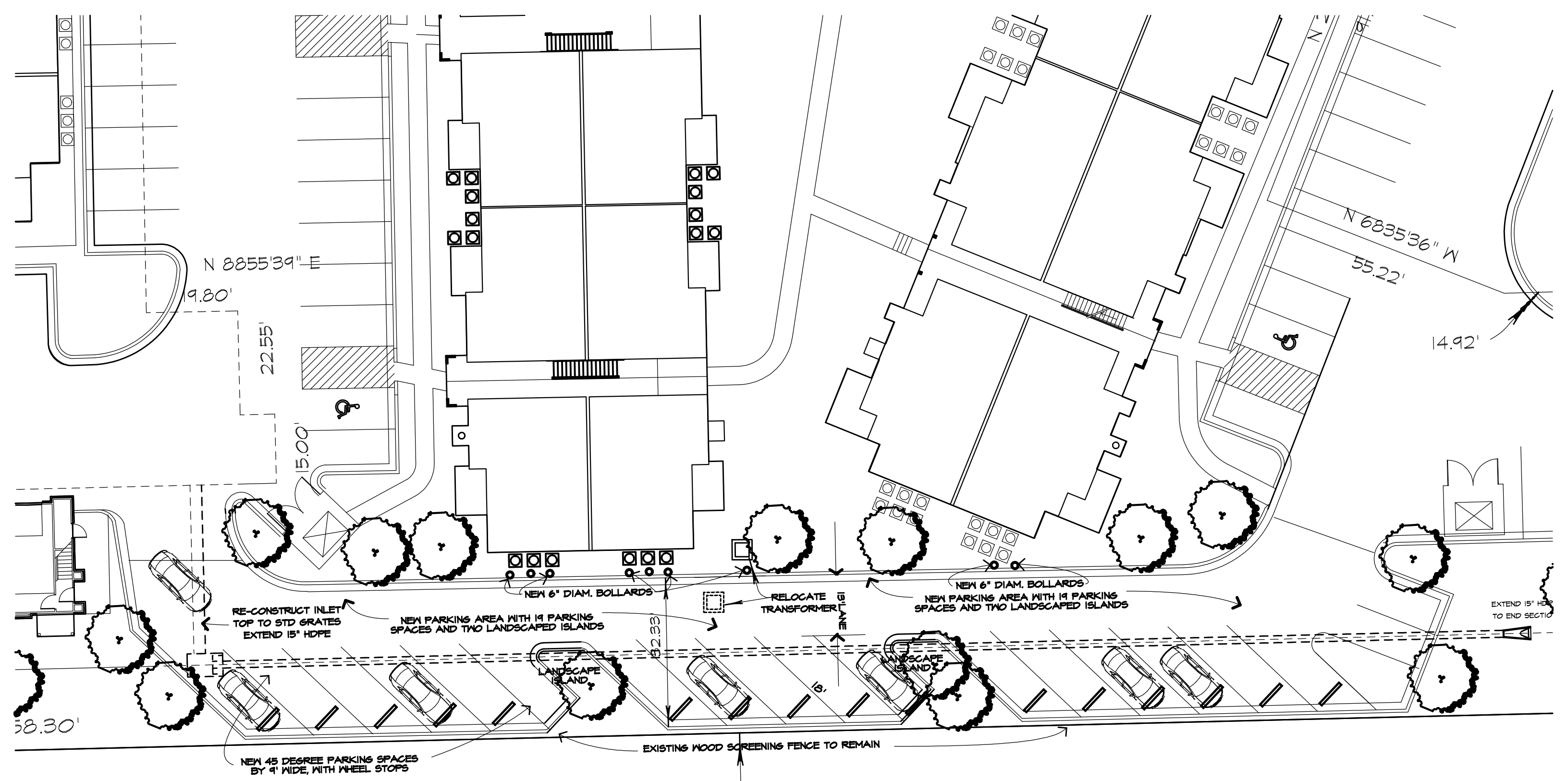
PARTIAL SITE PLAN FOR ADDITIONAL PARKING IN THE LANDSCAPE BUFFER 1" = 20'
