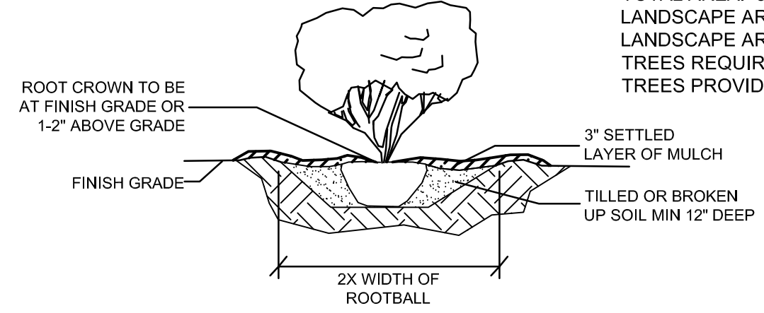
TYP. SHRUB PLANTING: NOT TO SCALE
