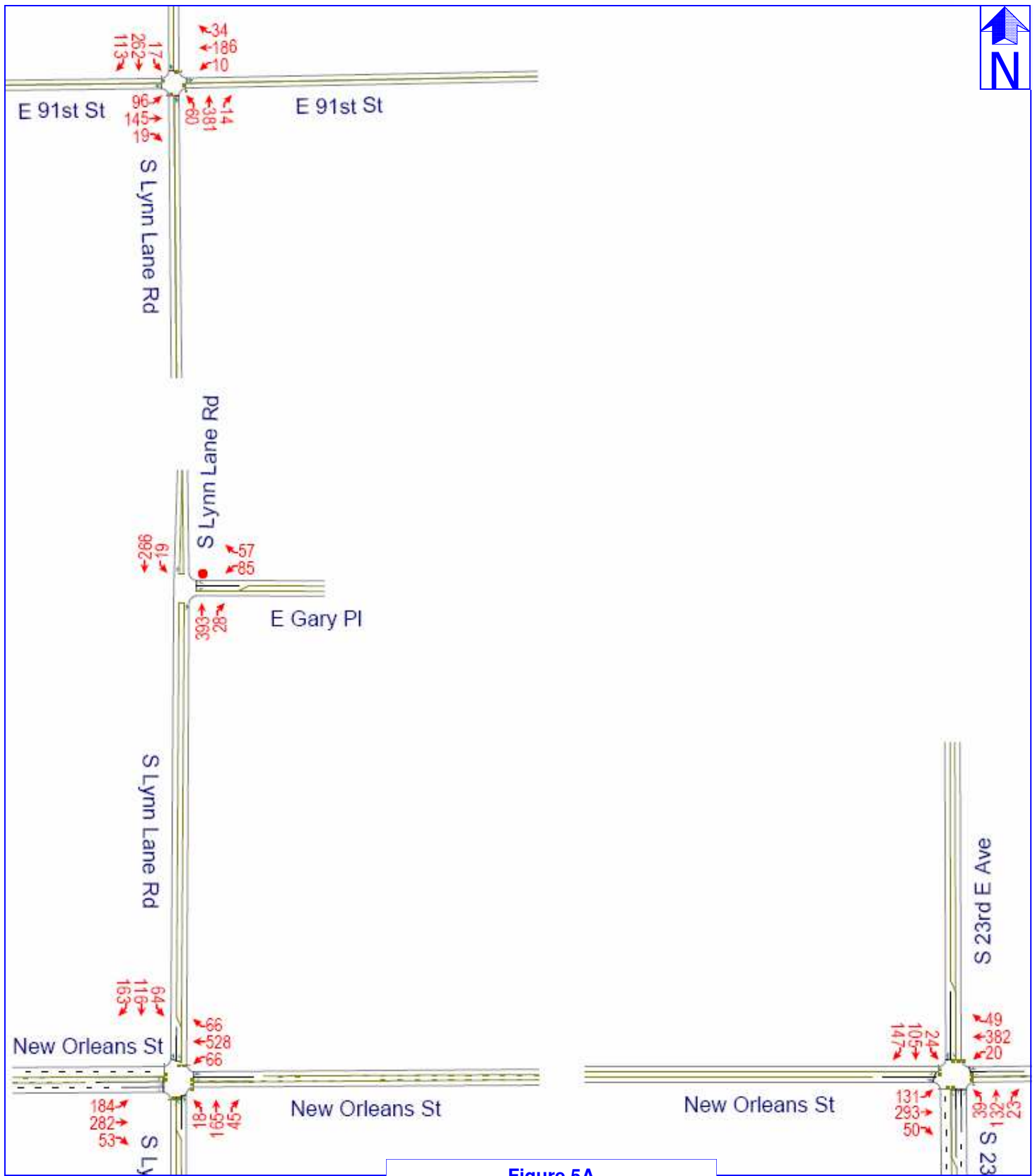
Figure 5A Projected 5-Year Traffic Volumes AM Peak Hour
